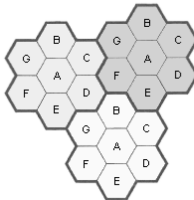
Cells with the same letter use the same set of frequencies.
