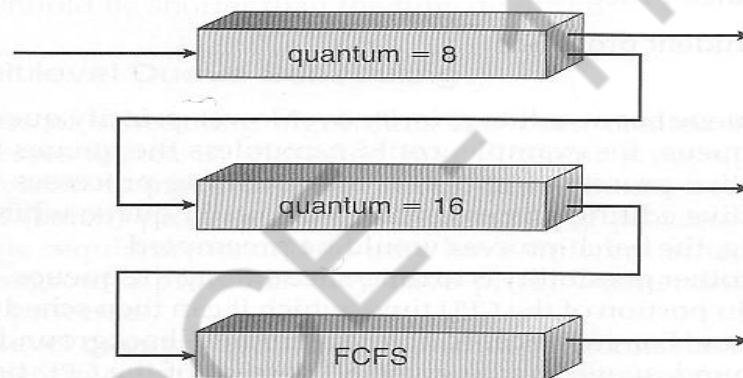
Figure Multilevel feedback queues.
