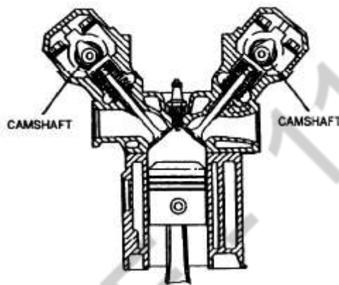
Figure 2-16.—Double overhead camshaft configuration.
